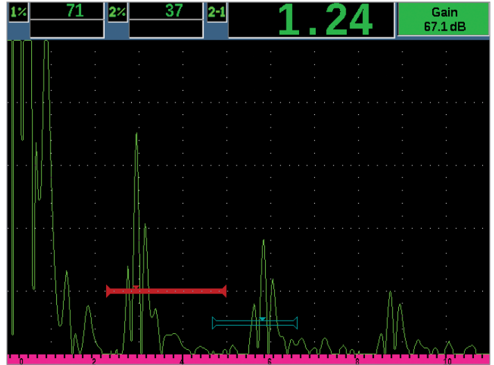
EPOCH 650 echo-to-echo with gate tracking
